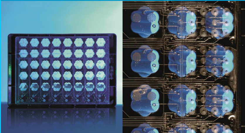
Microfluidic FlowerPlate ®
